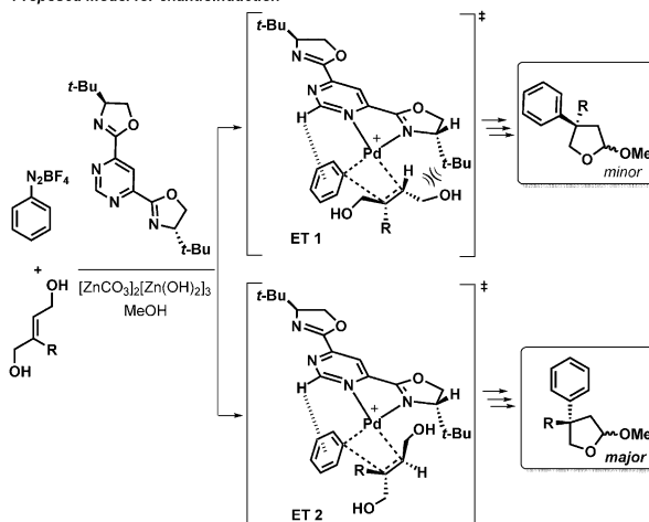
Scheme 4. Rationale for the enantioinduction in the Heck reactions.
