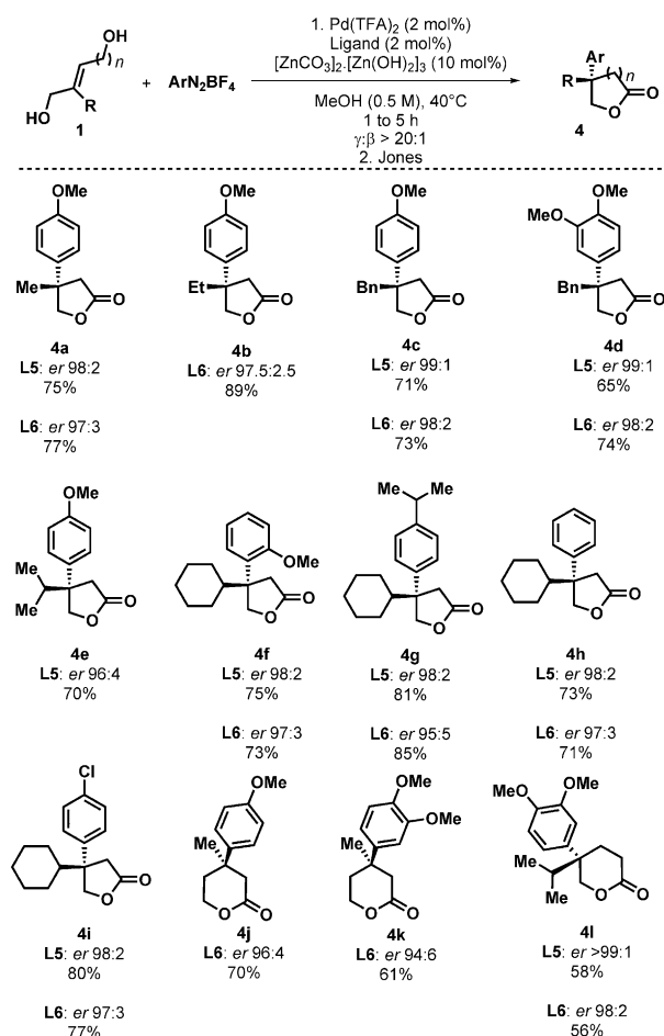
Scheme 3. Enantioselective synthesis of lactones 4.
