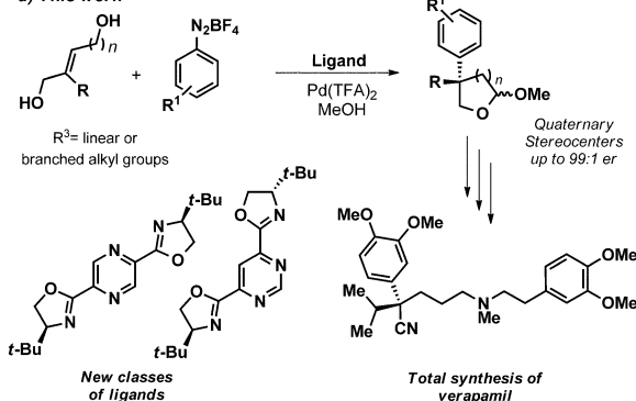
Scheme 1. Overview of enantioselective Heck reactions.
