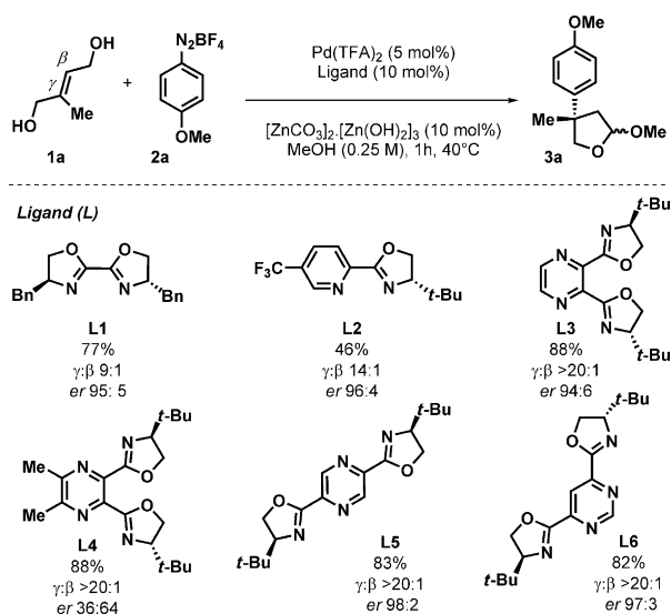
Scheme 2. Ligand screening for the enantioselective Heck reactions.
