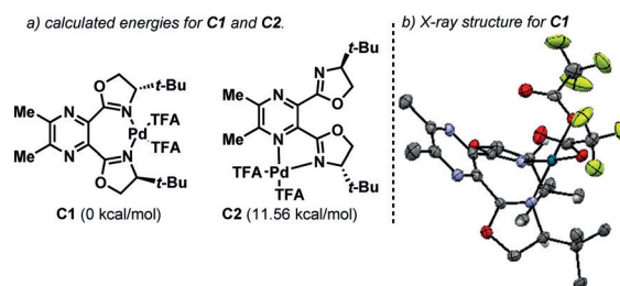
Figure 1. a) Energy profile for complexes C1 and C2 . b) X-ray structure of C1 . Ellipsoids set at 50% probability.
