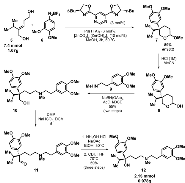
Scheme 5. Enantioselective synthesis of ( R )-verapamil ( 12 ).
